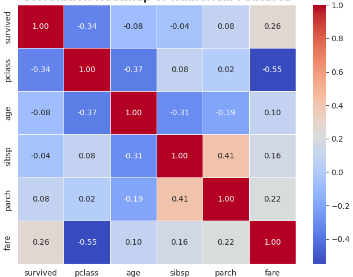
Correlation Heatmap of Numerical Features
